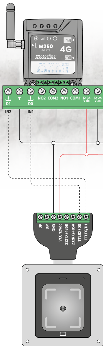
MQR340 WIEGAND READER (This reader is just an example)
