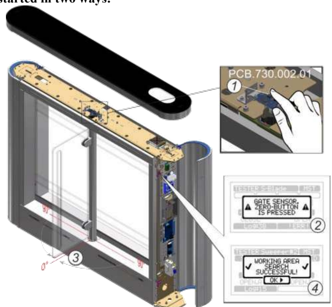
Fig.25 –Adjustment of the leaf zero position using the "zero" button
