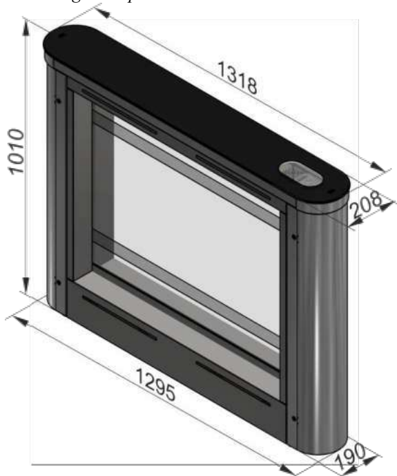
Fig. 4 – Overall dimensions of the turnstile cabinet
