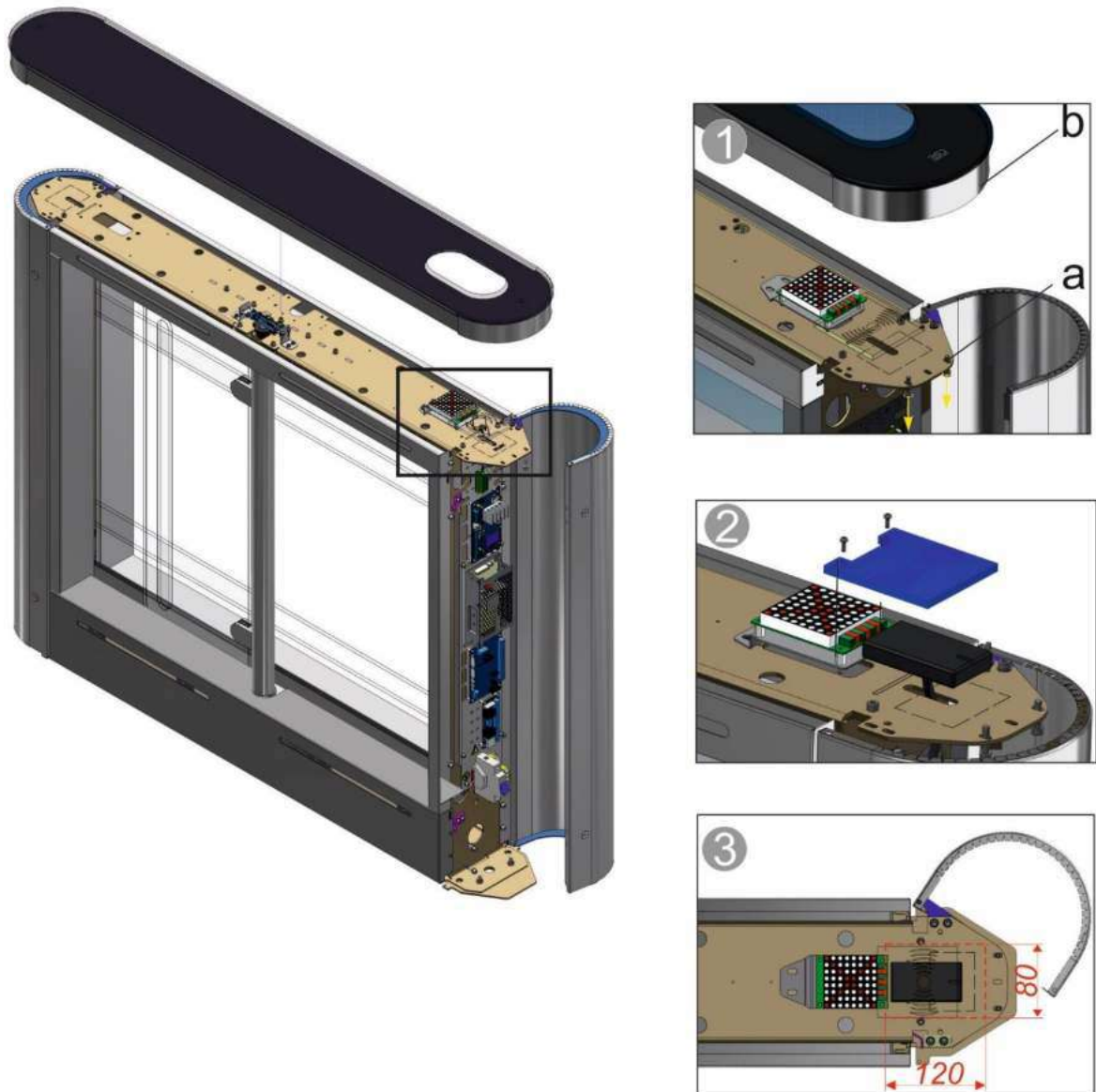
Fig.24 – Installation of card reader into the turnstile cabinet
