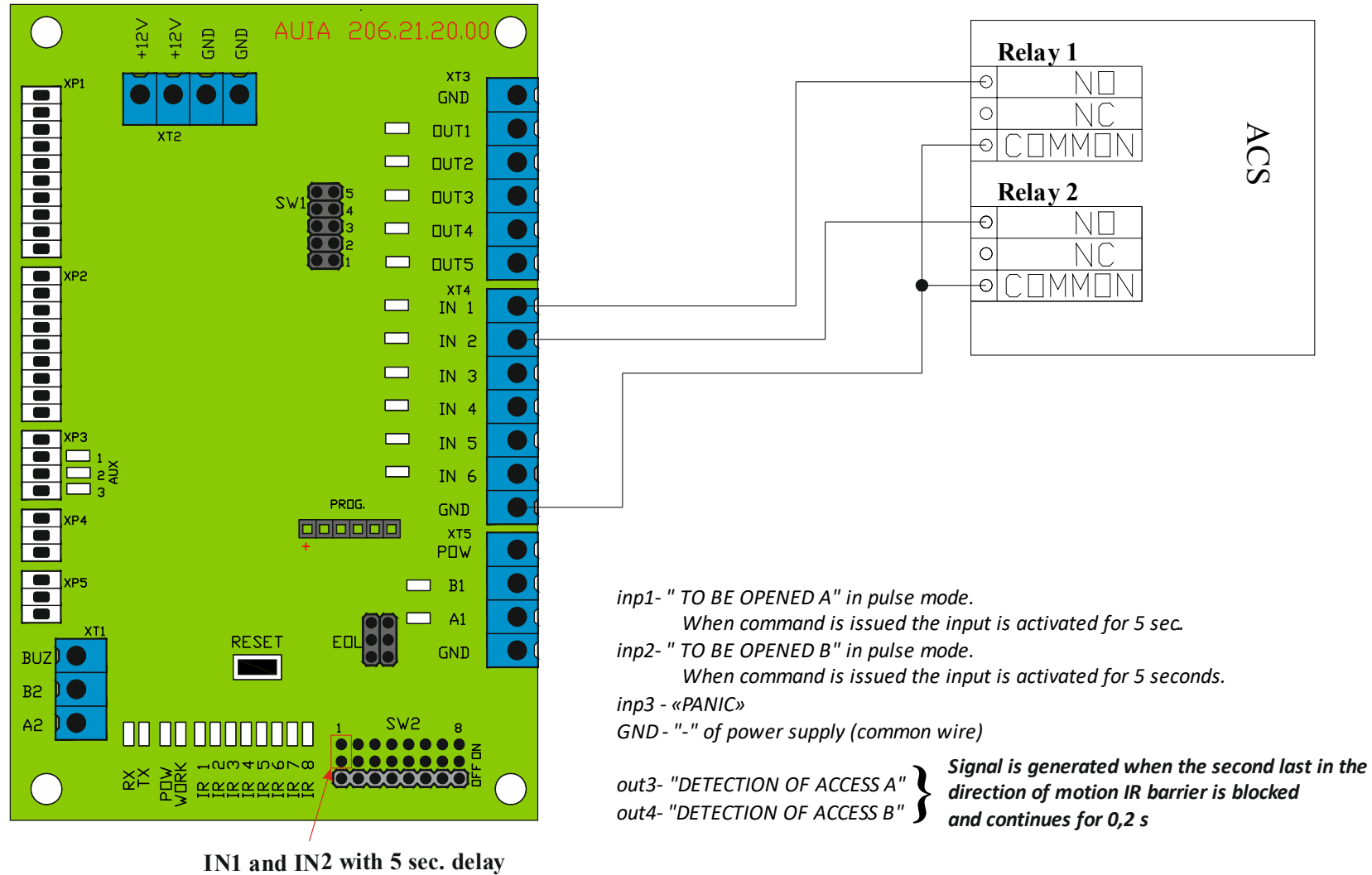
Annex E.2. Diagram of the turnstile connection to access control system (ACS)
