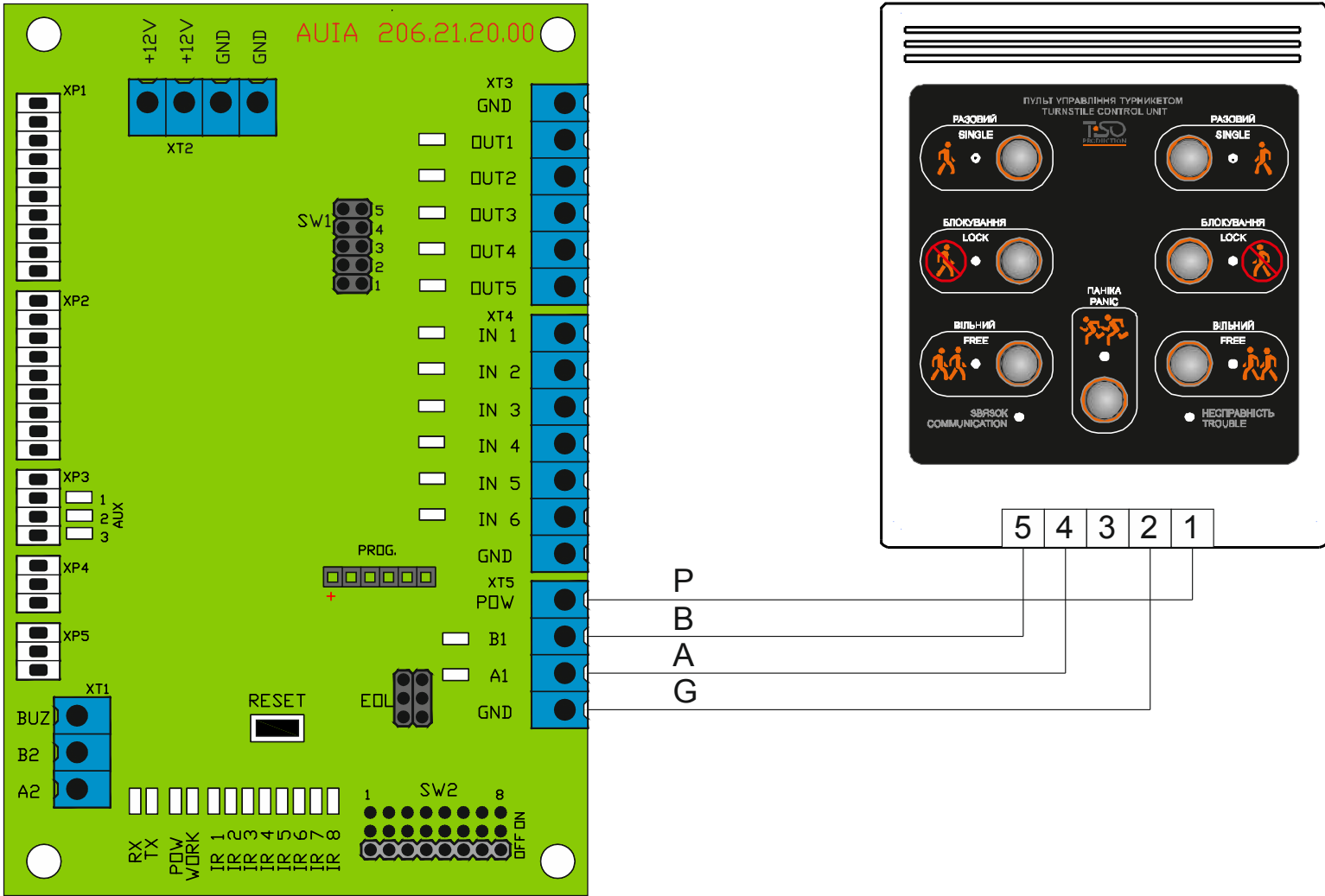
Annex E.4 Diagram of the turnstile connection to control panel
