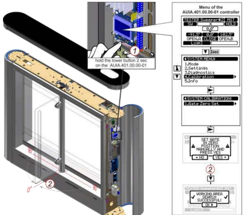
Fig.26 – Adjustment of the leaf zero position using the menu of controller AUIA.401.00.00-01
