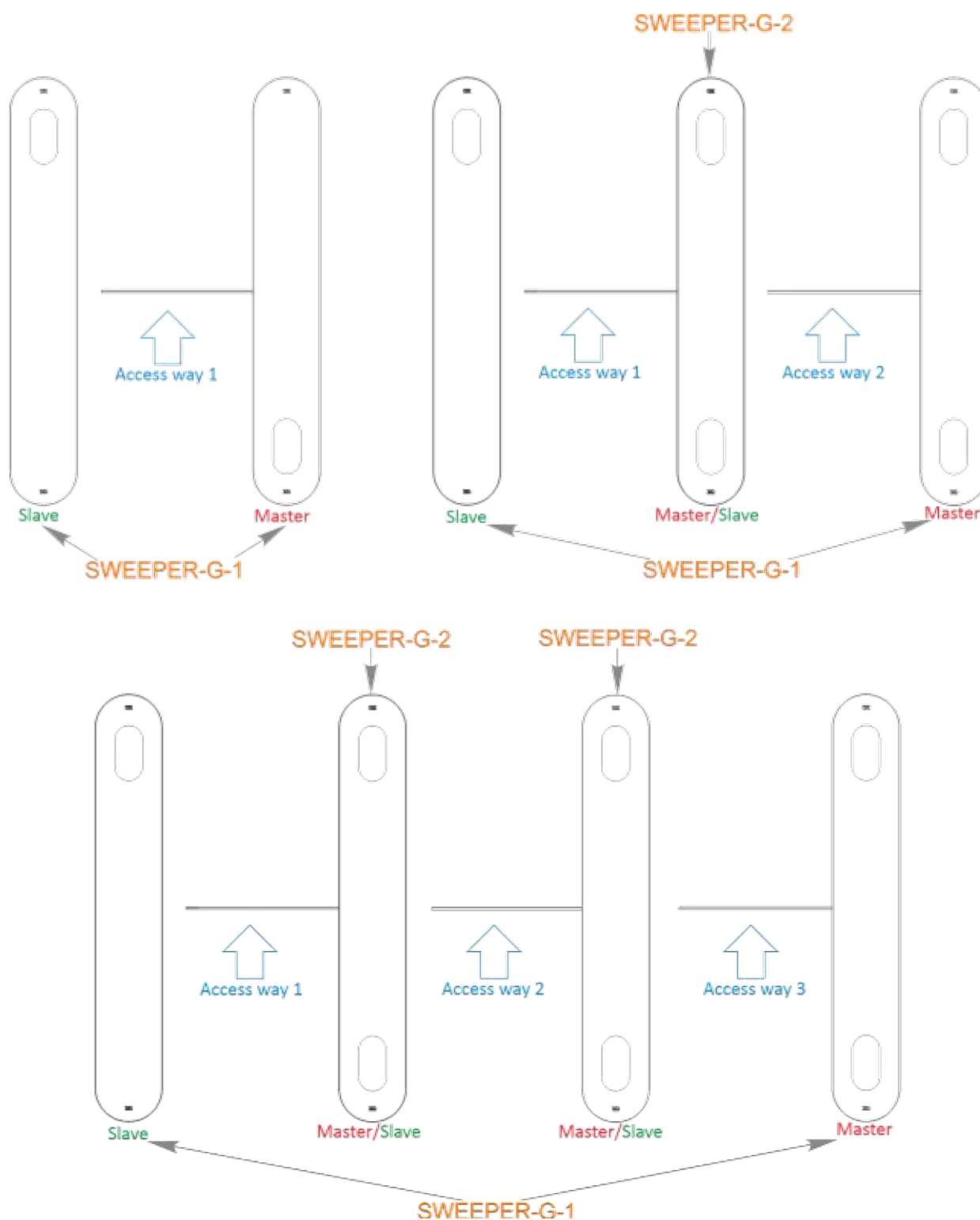
Fig. 16 – The "Sweeper-G-BM" turnstile lanes arrangement options
