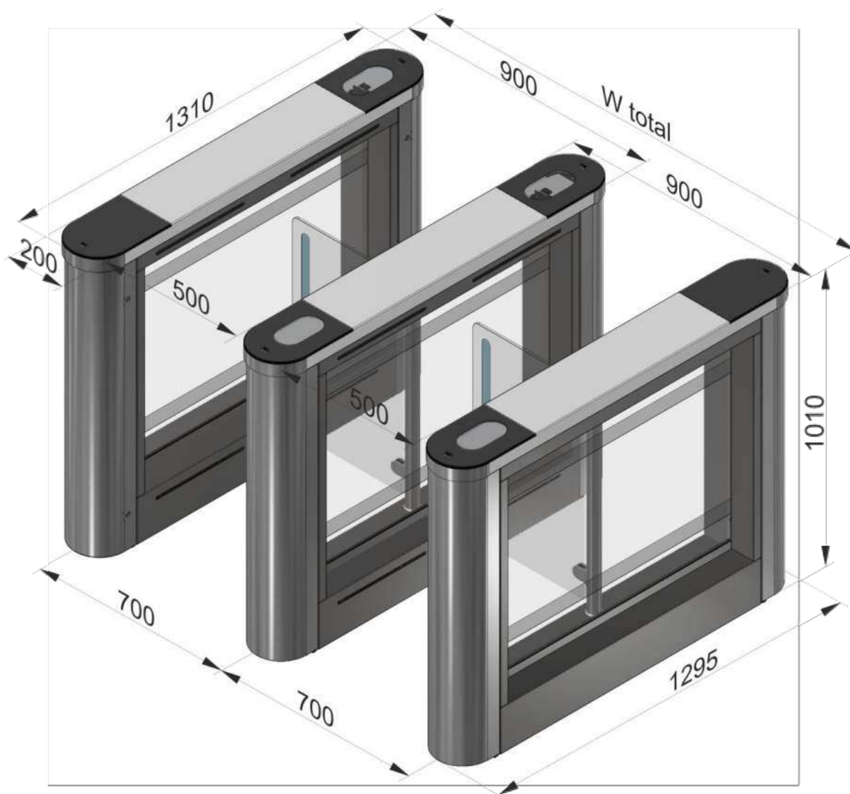
Fig. 3 – Dimensions of turnstile group
