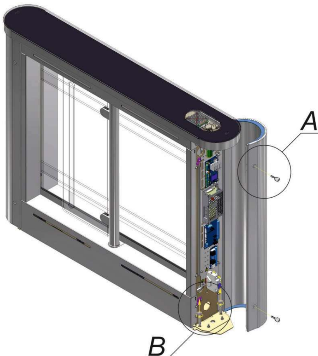
Fig. 17 – Turnstile dismantling and relocation from pallet
