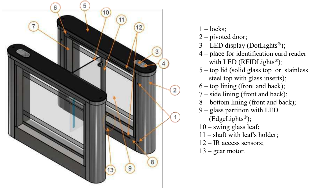
Fig. 5 – Design of single side cabinets type turnstile "Sweeper-G-BM-1" T3.KCD.XD
