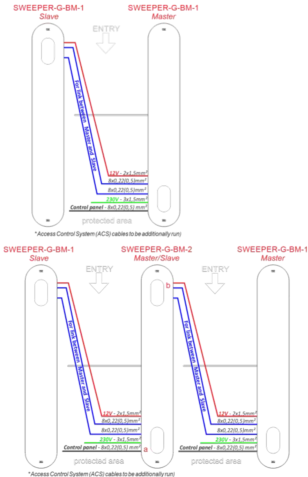
Fig. 19 – General view of connection between cabinets
