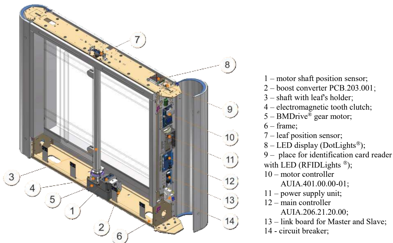
Fig. 7 – General appearance and design of “Sweeper-G-BM-1” turnstile mechanism (Master cabinet)
