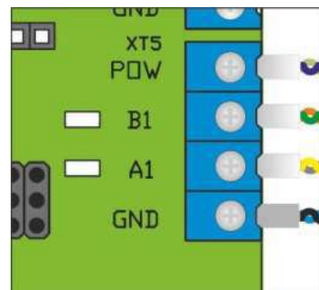
Fig. 23 – Connection of control desk link cable to terminals AUIA.206.21.20.00
