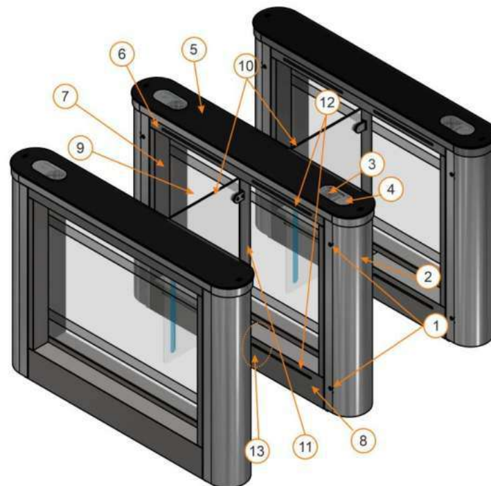
Fig. 6 – Design of the "Sweeper-G-BM-2" type turnstile T3.KCD.XD.X
