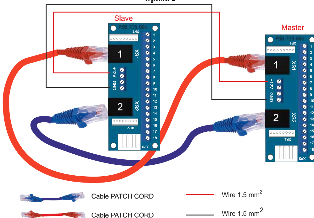
Fig. 20 – Options of cable connection between cabinets Master and Slave
